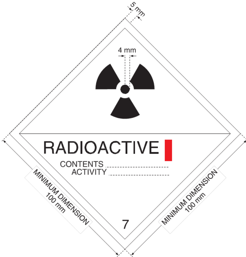
FIG 2. Category I-WHITE label. The minimum width of the line inside the edge forming the diamond shall be 2 mm. The background colour of the label shall be white, the colour of the trefoil and the printing shall be black, and the colour of the category bar shall be red.
