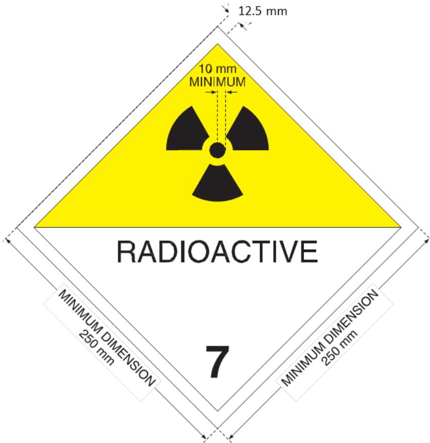
FIG 6. Placard. Except as permitted by para. 571, minimum dimensions shall be as shown; when different dimensions are used, the relative proportions shall be maintained. The number '7' shall not be less than 25 mm high. The background colour of the upper half of the placard shall be yellow and the lower half white, the colour of the trefoil and the printing shall be black. The use of the word "RADIOACTIVE" in the bottom half is optional, to allow the alternative use of this placard to display the appropriate UN number for the consignment.
