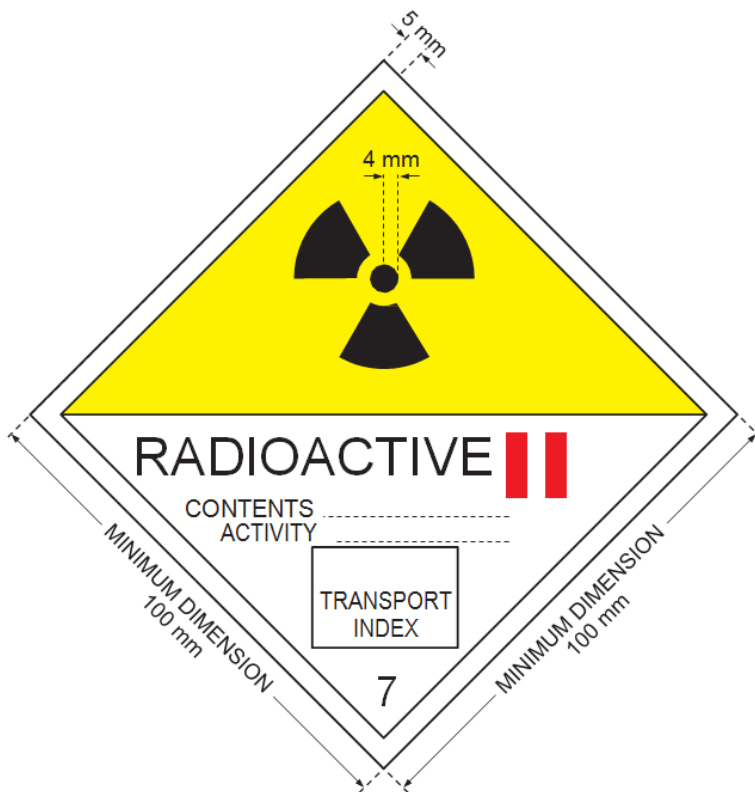
FIG 3. Category II-YELLOW label. The minimum width of the line inside the edge forming the diamond shall be 2 mm. The background colour of the upper half of the label shall be yellow and the lower half white, the colour of the trefoil and the printing shall be black, and the colour of the category bars shall be red.
