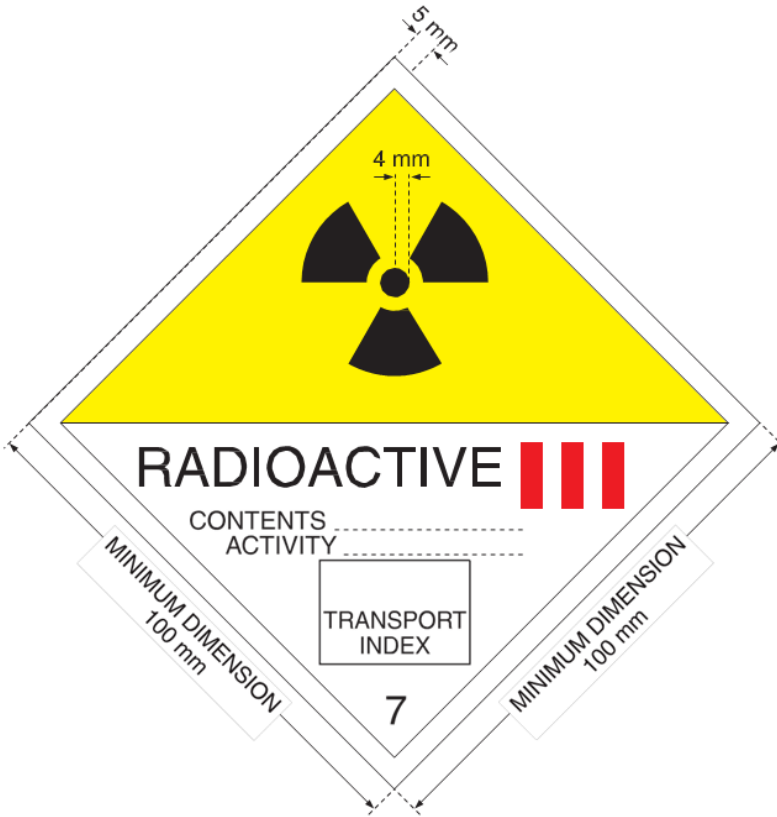
FIG 4. Category III-YELLOW label. The minimum width of the line inside the edge forming the diamond shall be 2 mm. The background colour of the upper half of the label shall be yellow and the lower half white, the colour of the trefoil and the printing shall be black, and the colour of the category bars shall be red.
